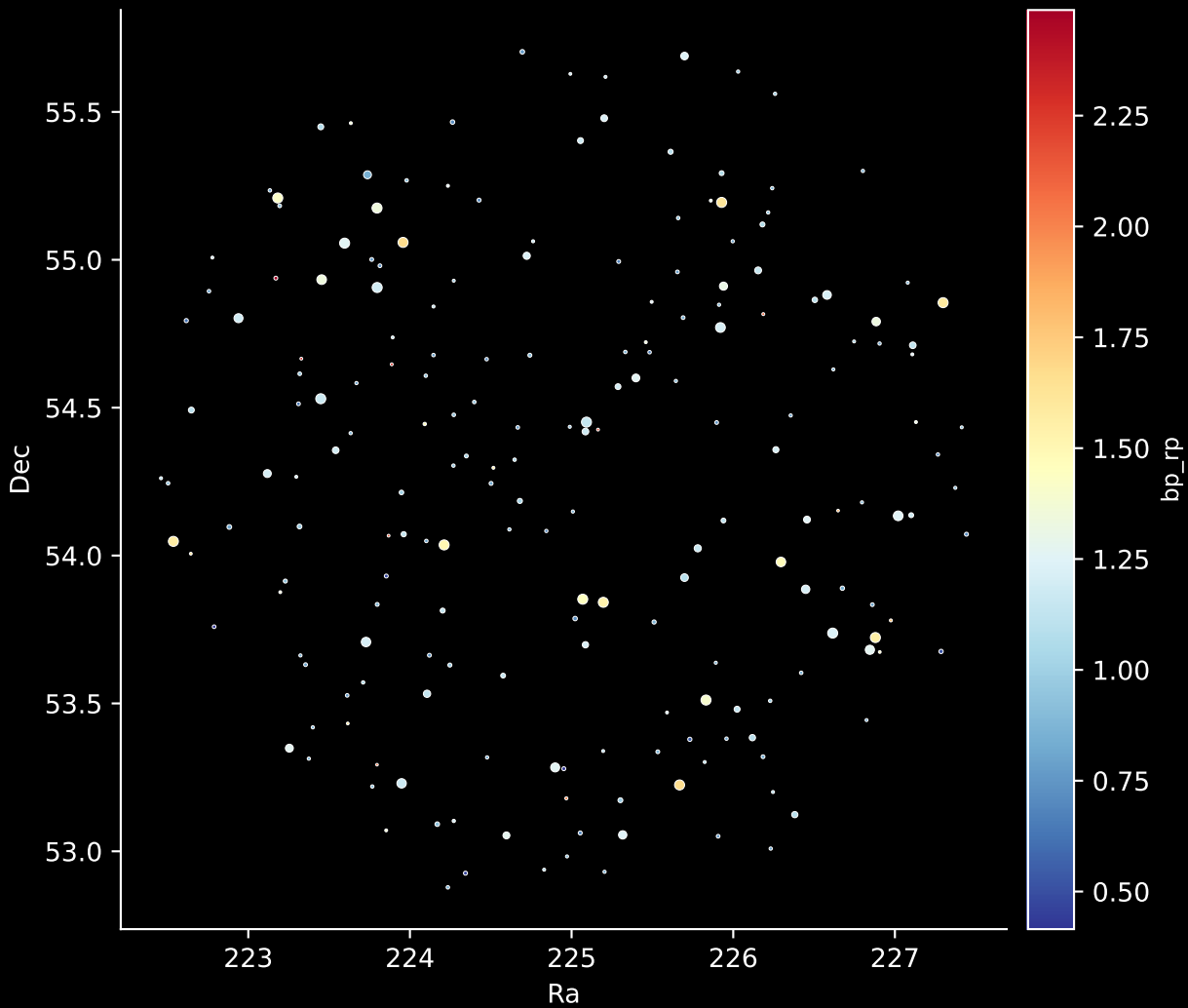
APOGEE DR17 Field: [164+34_MGA] Stars: 201
