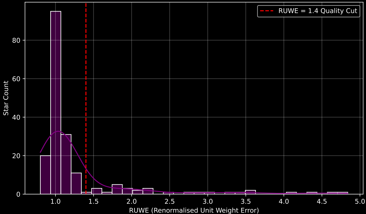
GAPOGEE DR17 Field [164+34_MGA] RUWE Distribution (n= 187)
