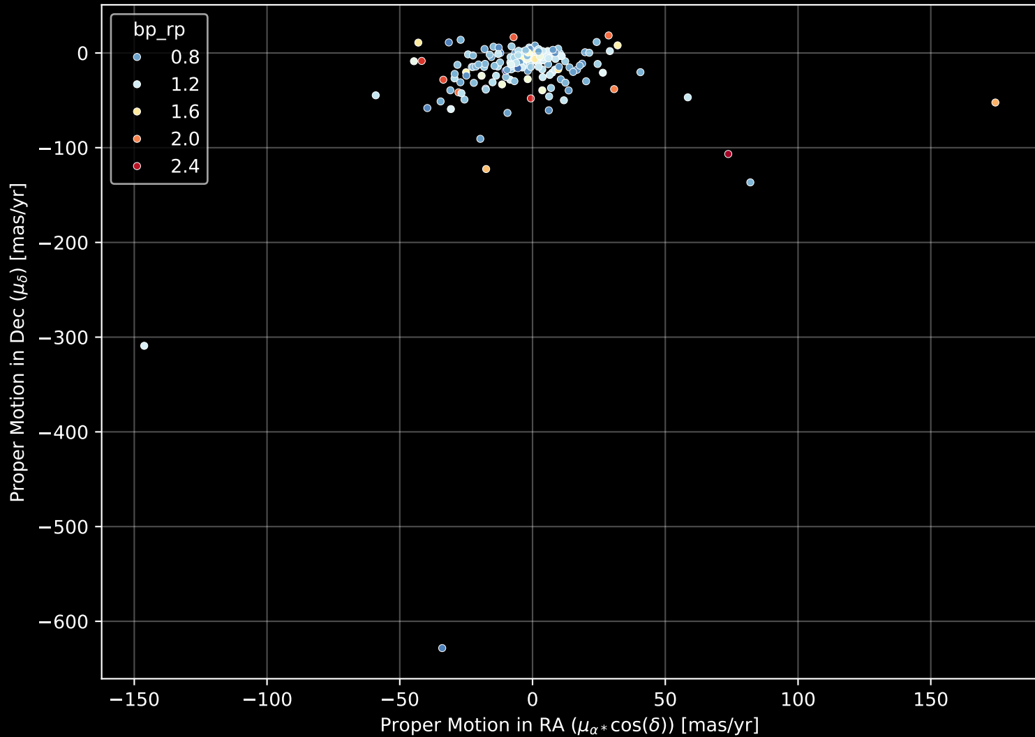
APOGEE DR17 Field: [164+34_MGA] Proper Motion Diagram (n= 201)
