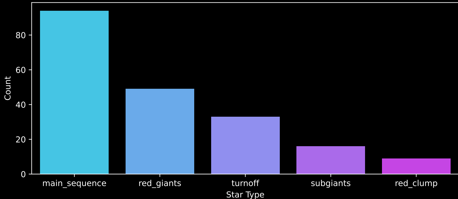
APOGEE DR17 Field: [164+34_MGA] Count plot of Star Type
