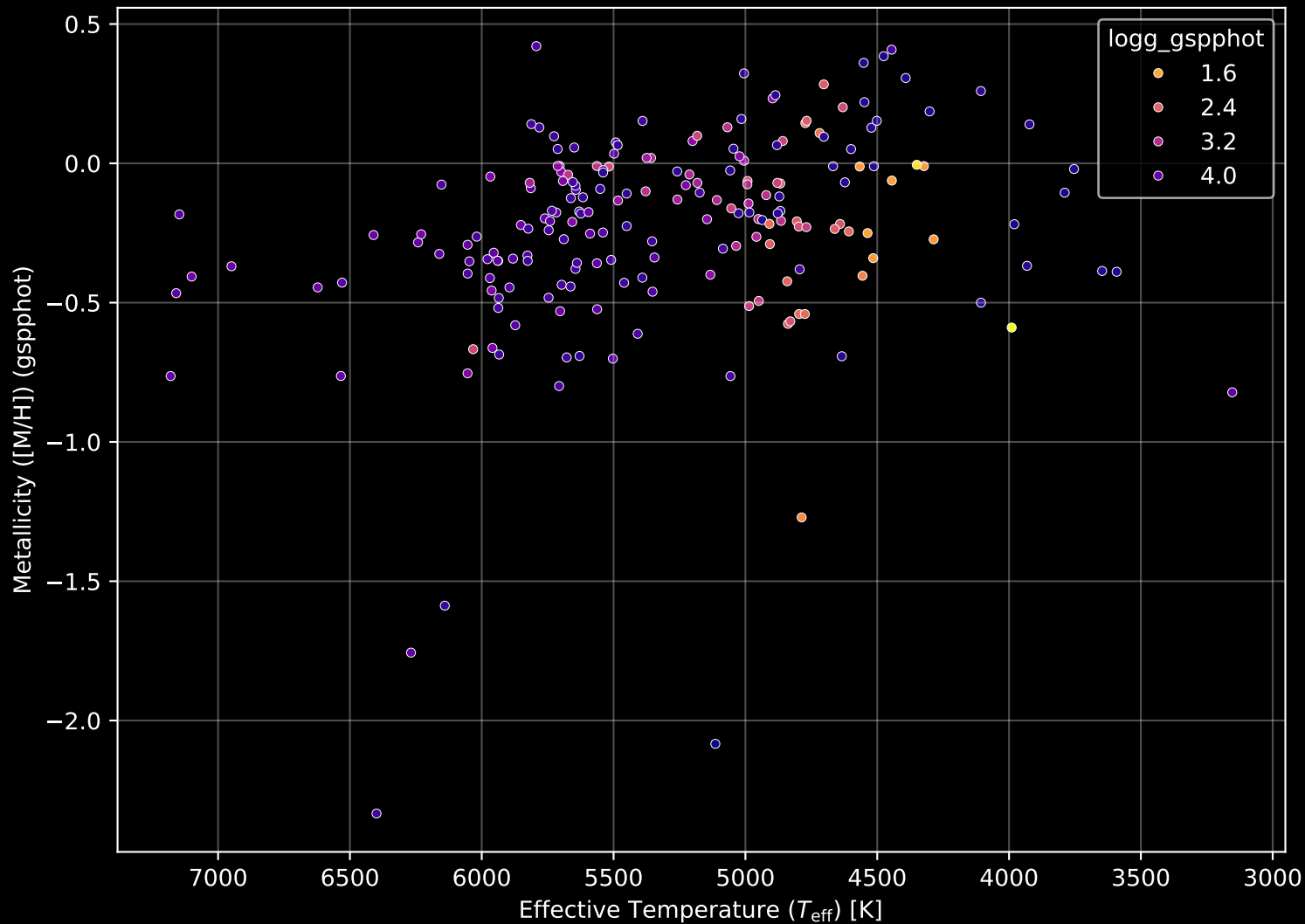
APOGEE DR17 Field: [164+34_MGA] Stellar Population Parameters (n= 201)
