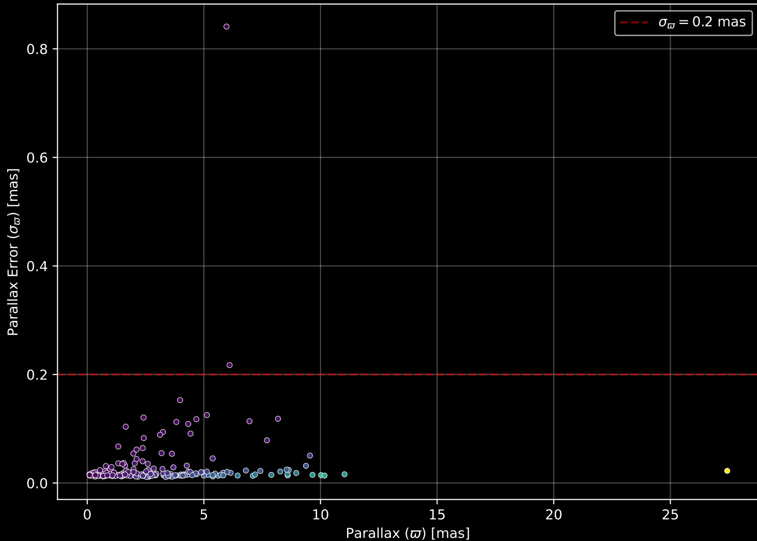
APOGEE DR17 Field: [164+34_MGA] Parallax Quality (n= 201)
