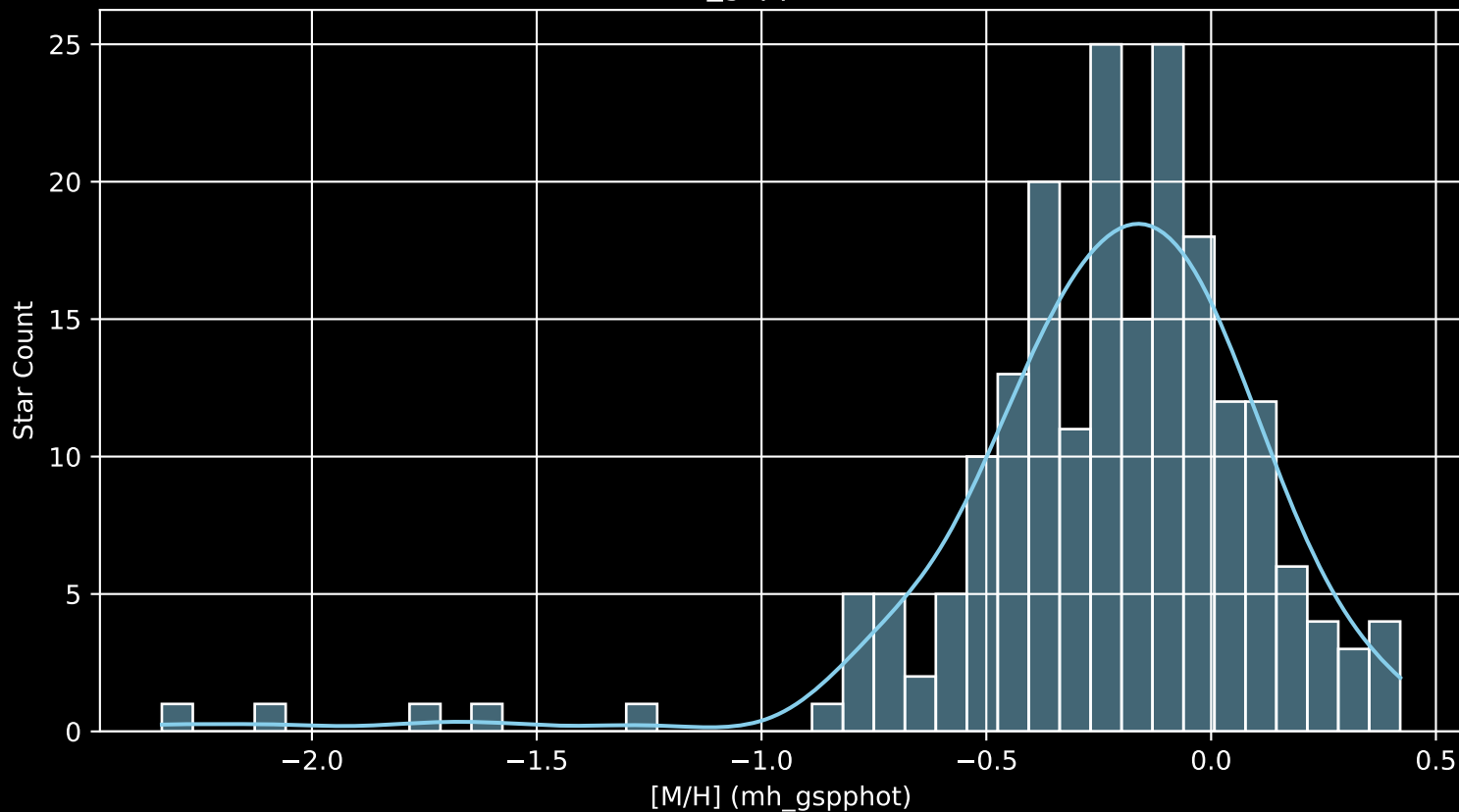
APOGEE DR17 Field: [164+34_MGA [M/H] (mh_gspphot) (n= 201)
